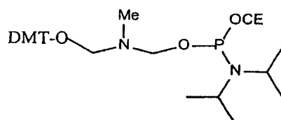
Neutral Phosphoramidite
